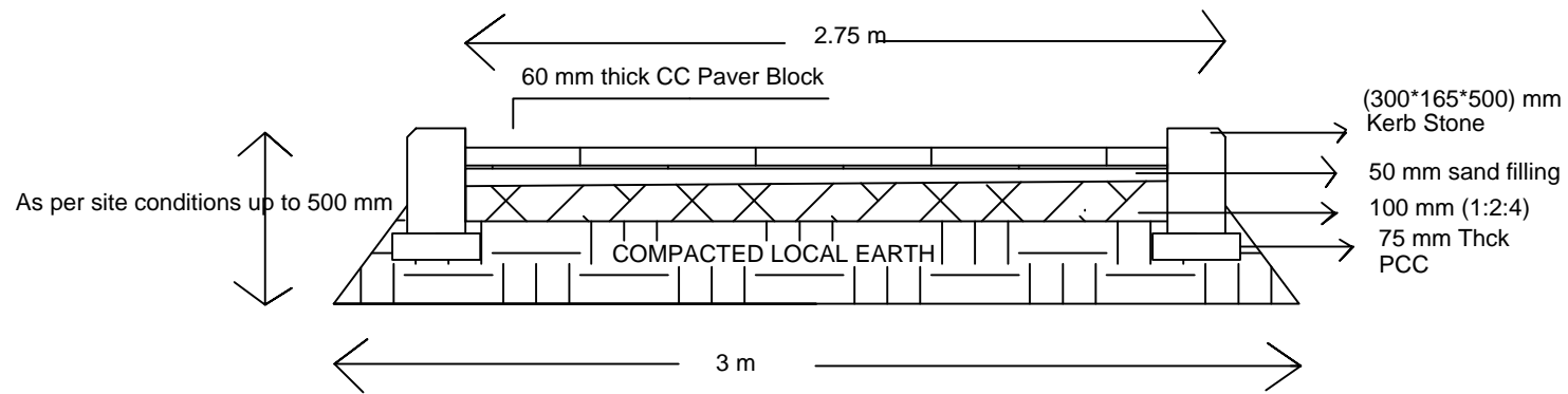
Typical Section of C.C Paver Block Pathway for 26 mtrs and 30 mtrs R.O.W
